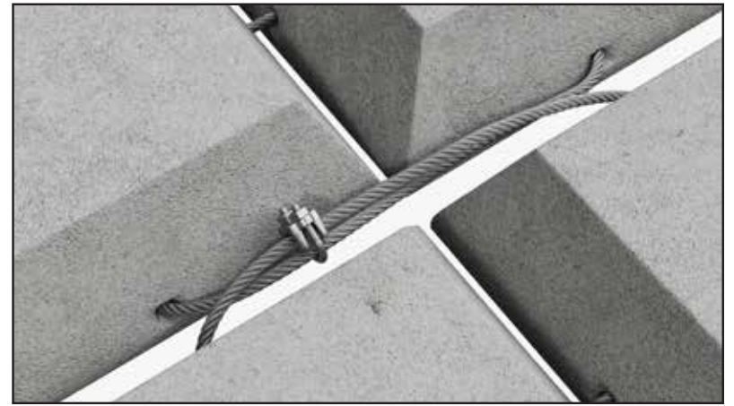
Articulated Concrete Cable Block Mats are joined together with Cable Clamps
